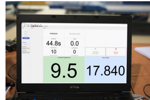
Program interface
