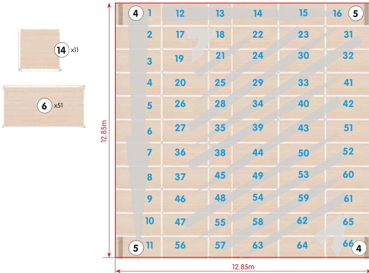
Figure 3 - Arrangement and order of the panels assembly
