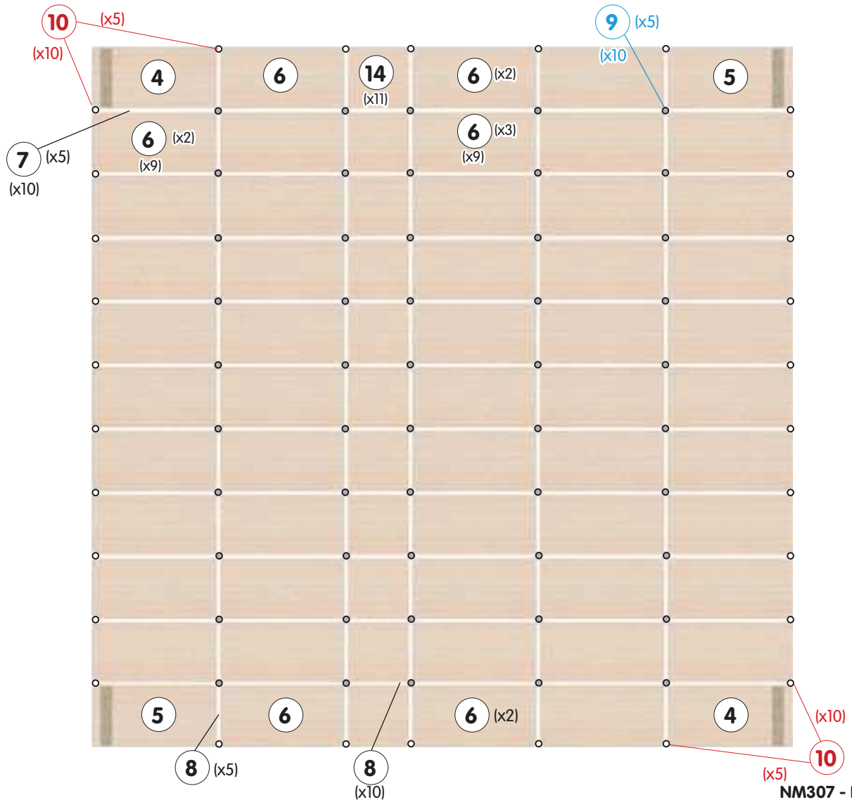
Figure 8 - Distribution of floor panels and connecting parts
