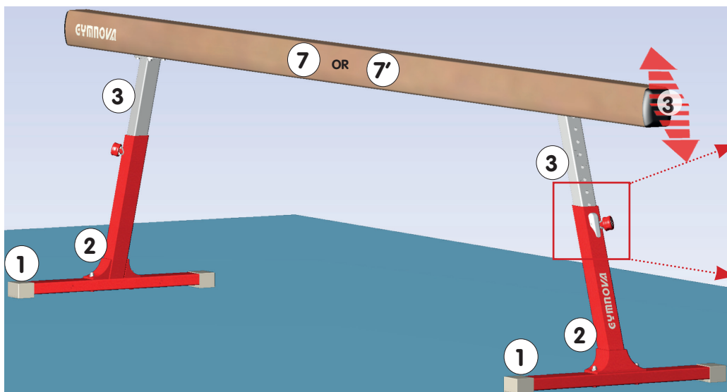
Figure 14 - Side view 5.04m or 5.01m
